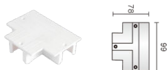
T CONNECTOR RECESSED COVER
