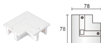
L CONNECTOR RECESSED COVER
