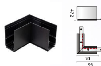
L DEEP CONNECTOR-FLAT RIGHT
