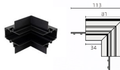
L RECESSED CONNECTOR-STEREO
