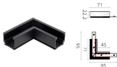
L CONNECTOR-FLAT RIGHT
