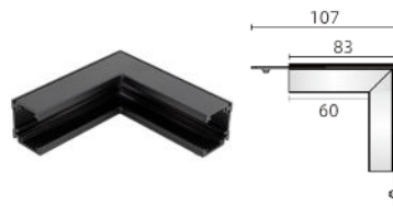
L CONNECTOR-STEREO
